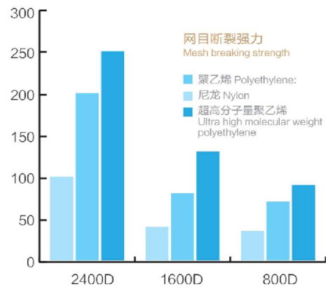
水产养殖业常用网衣网目断裂强力对比 Comparison of breaking strength of net mesh in aquaculture industry
